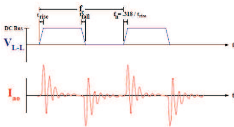
Noise Source: Drive Induced Common Mode Current
